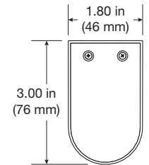
Shade Bracket
